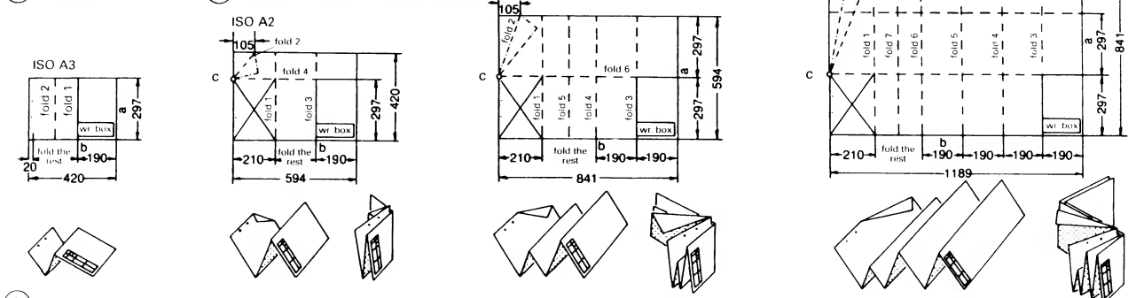
⑧ Dimensions and scheme for folding
